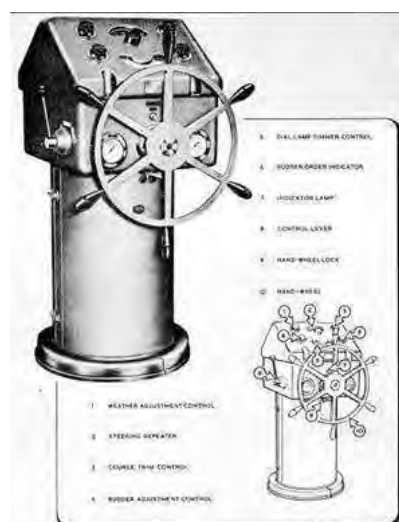
FIG. 2.1. Bridge control unit
